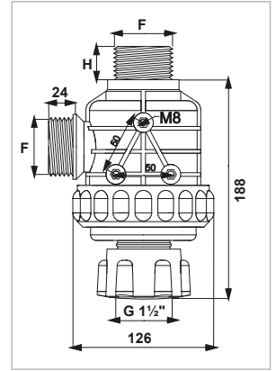
Çek Valf Kiti Shut-off Valve Válvula de cierre
